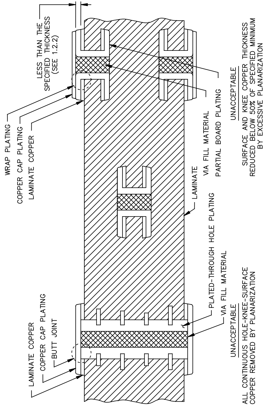
FIGURE 9. Unacceptable plated-through hole wrap plating (continuous hole-knee-surface copper plating).
