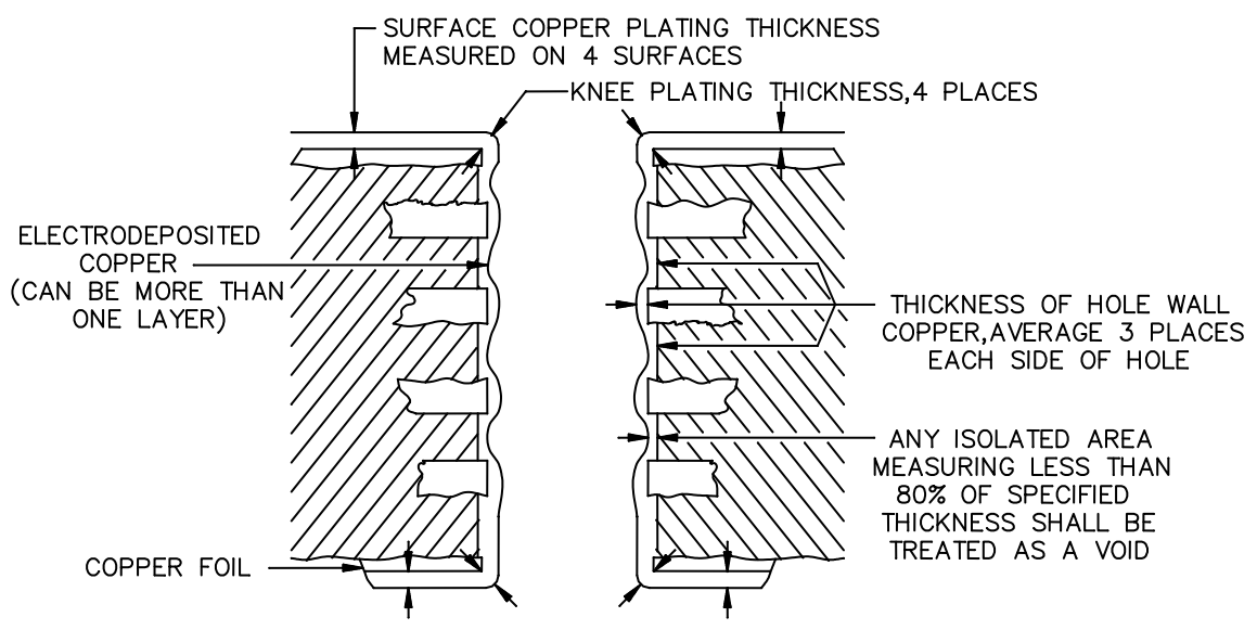
FIGURE 7. Copper plating thickness.
